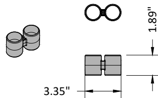
SIDE PLATE TO BE INSTALLED ON THE PERIMETER OF THE SYSTEM
